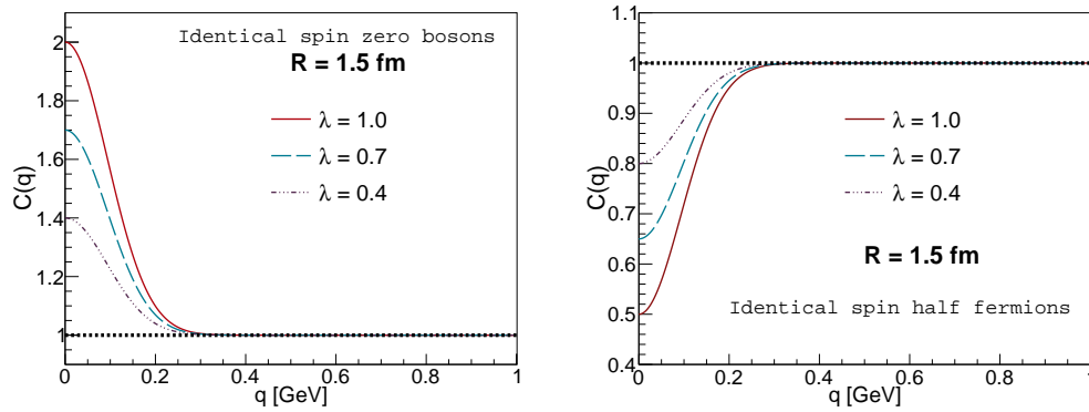
Figure 3.6: Correlation as a function of q using different \lambda values: 1 (red solid line), 0.7 (blue dashed line) and 0.4 (purple dot-dashed line) for quantum statistics cases: bosons with spin zero (left) and fermions with spin half (right).
