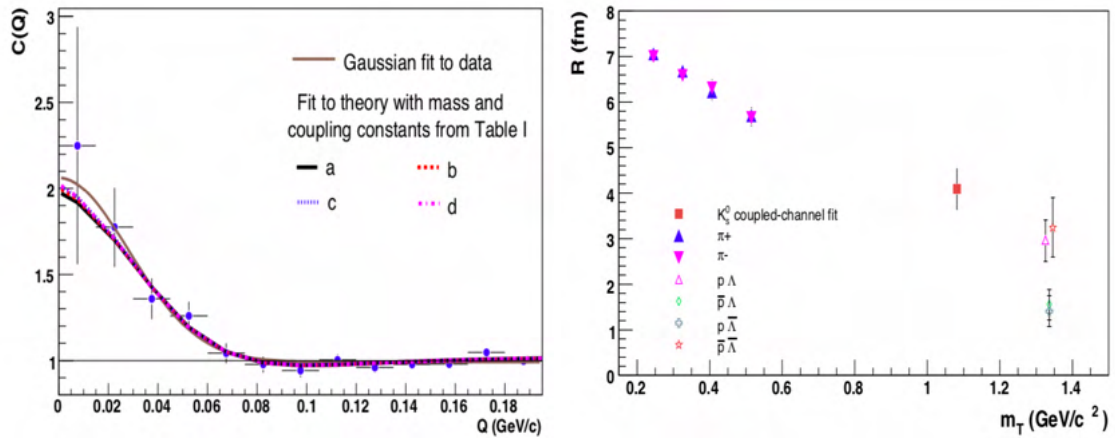
Figure 3.11: Measurement of K_S^0 K_S^0 femtosopic correlations from STAR Collaboration in AuAu collisions with \sqrt{s_{NN}} = 200 GeV. More information in the text. Extracted from [203].
