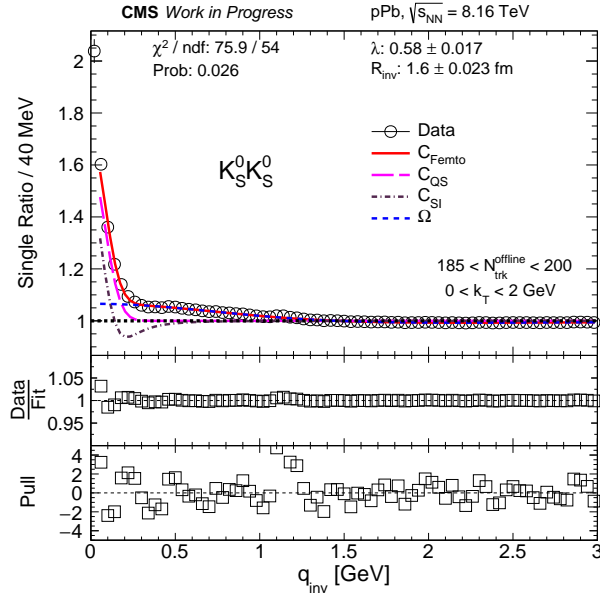
Figure 6.1: Single ratio of K_S^0 K_S^0 pairs as a function of q_{inv} (black open circles) integrated in k_T ( 0 < k_T < 2 GeV) and multiplicity range ( 185 < N_{trk}^{offline} < 200 ). The fit is performed using Eq. (5.10), where the full fit (red solid line), the Bose-Einstein quantum statistic term (pink long dashed line), the strong FSI (purple dash-dotted line) and the non-femtoscopic background (blue short dashed line) are shown. The parameters extracted from the fit, including only statistic uncertainties, fit quality ( \chi^2/ndf ), data/fit ratio and pull distributions are shown in the plot. More informations in the text.
