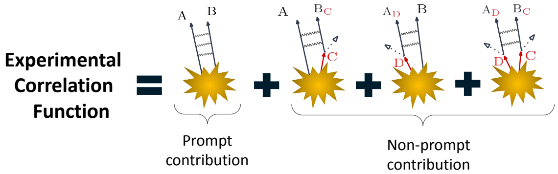
Figure 5.25: Sketch of the total correlation function as the sum of the prompt and non-prompt contributions. See details in the text. 12
