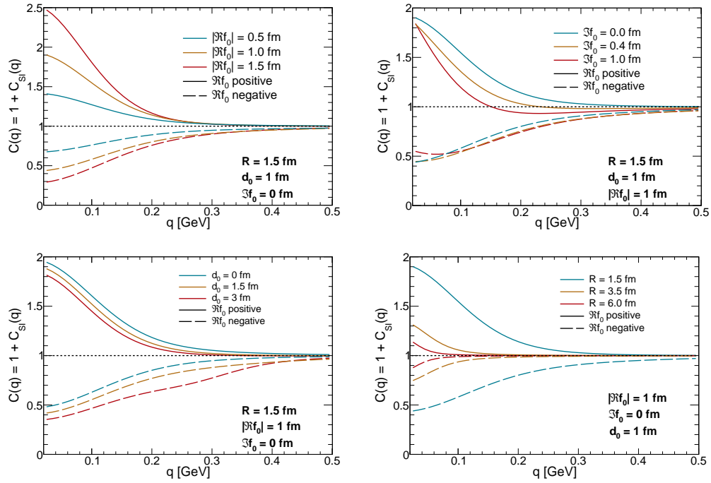
Figure 3.9: Example of the contribution of the strong FSI parameters using the LL model, in Eq. (3.43), in the correlation function C(q) = 1 + C_{SI}(q) , for different values (in different colors) of \Re f_0 (top left), \Im f_0 (top right), d_0 (bottom left) and R (bottom right). The plots show results for both \Re f_0 > 0 fm (solid lines), and \Re f_0 < 0 fm (dashed lines). More information in the text.
