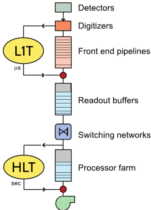
Figure 4.12: Schematical view of the CMS trigger system. Extracted from [301].
