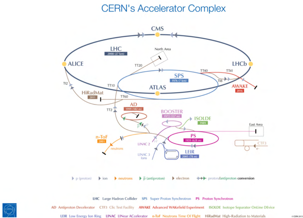
Figure 4.1: Schematic view of the CERN accelerator complex. Extracted from https://cds.cern.ch/record/1621583 [last access on 13/Mar/2021].
