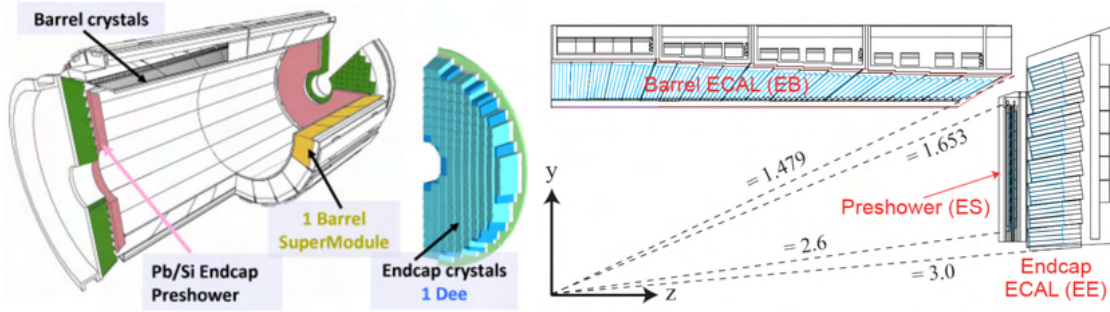
Figure 4.8: Representation of the ECAL sections, on the left. Extracted from [296]. Geometrical view of the ECAL in the zy plane with \eta ranges included, on the right. Extracted from [297].
