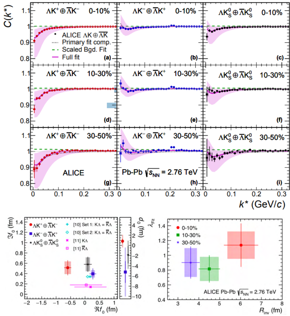
Figure 3.13: Top panel: measured correlation as a function of k^* ( q/2 ) for different K\Lambda pairs (solid circles) in PbPb collisions at \sqrt{s_{\text{NN}}} = 2.76 TeV, in three different centralities: 0-10% (top), 10-30% (middle) and 30-50% (bottom). The fit results (pink solid line), background (green dashed line), strong FSI only (black dotted line) and systematic uncertainties (pink band) are also shown. Bottom panel: the scattering quantities ( \Re f_0 , \Im f_0 , d_0 ) measured using the LL fit are shown on the left, while the \lambda versus R_{\text{inv}} results are shown on the right. Extracted from [232].
