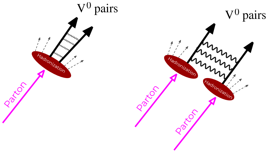
Figure 5.20: Schematic view of the V^0 pair production from a single parton (left) and from two partons (right). See more details in the text.
