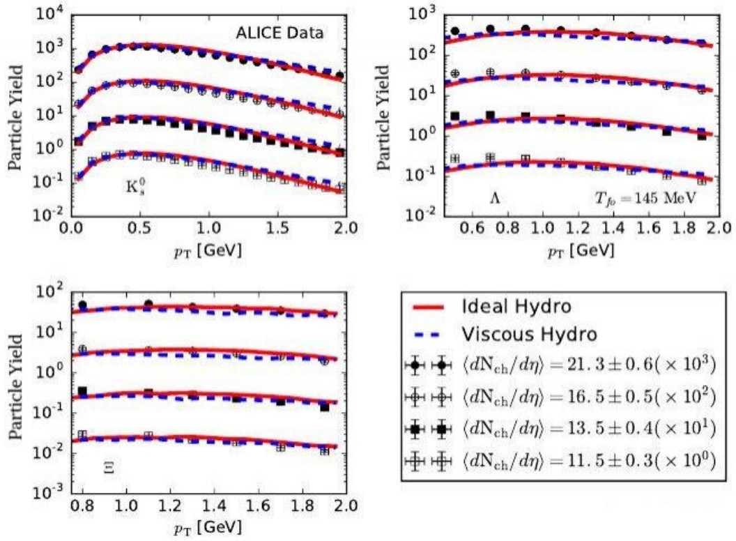
Figure 2.19: Particle yield versus p_T of strange particles: K_S^0 (top left), \Lambda + \bar{\Lambda} (top right) and \Xi^- + \bar{\Xi}^+ (bottom left) as measured by ALICE collaboration [102] (markers), compared with hydrodynamical simulations from the CHES code [75] in four ranges of multiplicity, as shown in the legend. Lines represent hydrodynamical calculations for ideal (red solid line) and viscous (blue dashed line) cases with freezeout temperature of T_{fo} = 145 \text{ MeV} .
