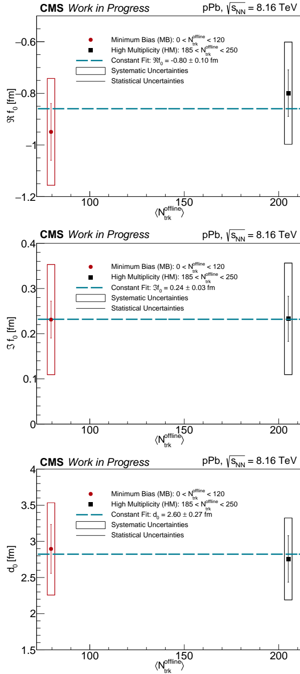
Figure 6.9: Scattering parameters \mathcal{R}f_0 (top), \mathcal{S}f_0 (middle) and d_0 (bottom), as a function of multiplicity, for minimum bias (red circle), 0 < N_{\text{trk}}^{\text{offline}} < 120 , and high multiplicity (black square), 185 < N_{\text{trk}}^{\text{offline}} < 250 , samples. The blue-dashed line represents a constant fit. Both statistical (lines) and systematic uncertainties (boxes) are shown. More informations in the text.
