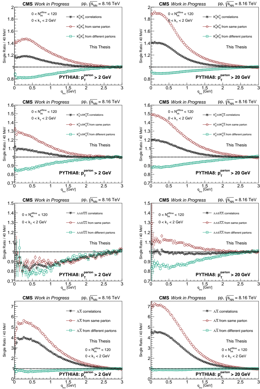
Figure 5.21: Single ratios as function of q_{inv} calculated using PYTHIA8 , in two different regimes: p_T^{\text{parton}} > 2 GeV (left panel) and p_T^{\text{parton}} > 20 GeV (right panel); for K_S^0 K_S^0 (top panel), K_S^0 \Lambda \oplus K_S^0 \bar{\Lambda} (middle-top panel), \Lambda \Lambda \oplus \bar{\Lambda} \bar{\Lambda} (middle-bottom panel) and \Lambda \bar{\Lambda} (bottom panel). The usual correlations (black open star) are compared with the cases where V^0 comes from same (open green circles) and different (open green squares) partons.
