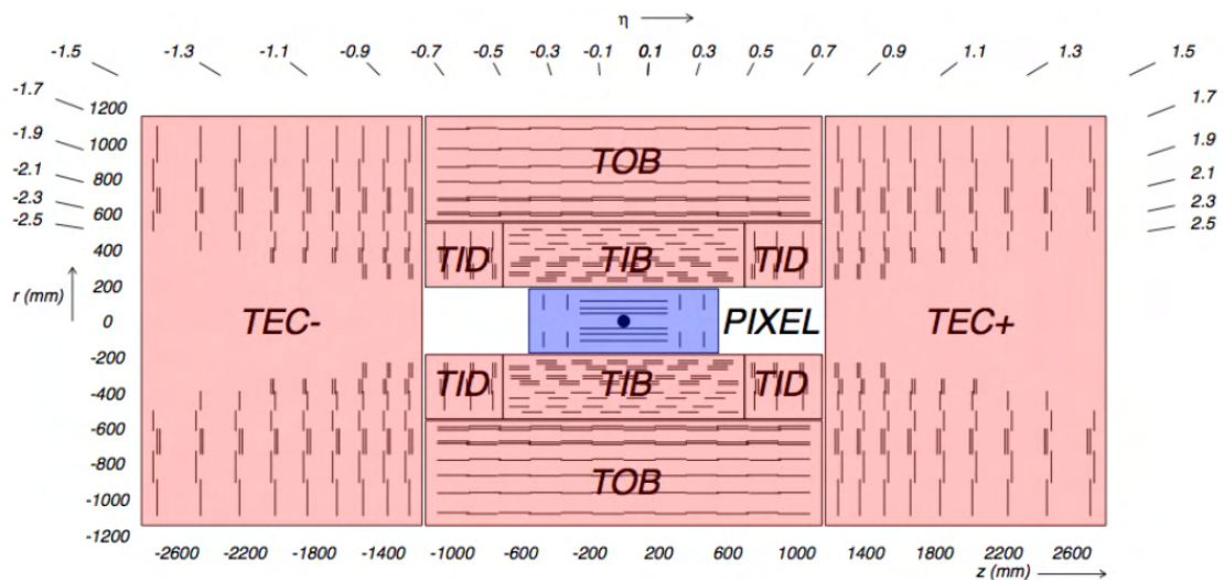
Figure 4.6: Geometrical view of CMS tracker systems in the zr plane with pixel (blue) and strip (red) components with lines representing the layers. The pseudorapidity range is also shown. Extracted from [4].
