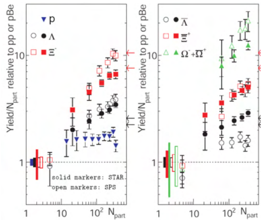
Figure 2.10: Production yield of protons and strange baryons ( \Lambda , \bar{\Lambda} , \Xi^- , \bar{\Xi}^+ and \Omega^- + \bar{\Omega}^+ ), measured by STAR collaboration in AuAu collisions at \sqrt{s_{NN}} = 200 GeV (solid markers) relative to the same yield in pp collisions and for NA57 collaboration in PbPb collisions at \sqrt{s_{NN}} = 17.3 GeV (open markers) relative to the same yield in pBe collisions as function of N_{part} . Extracted from [101].
