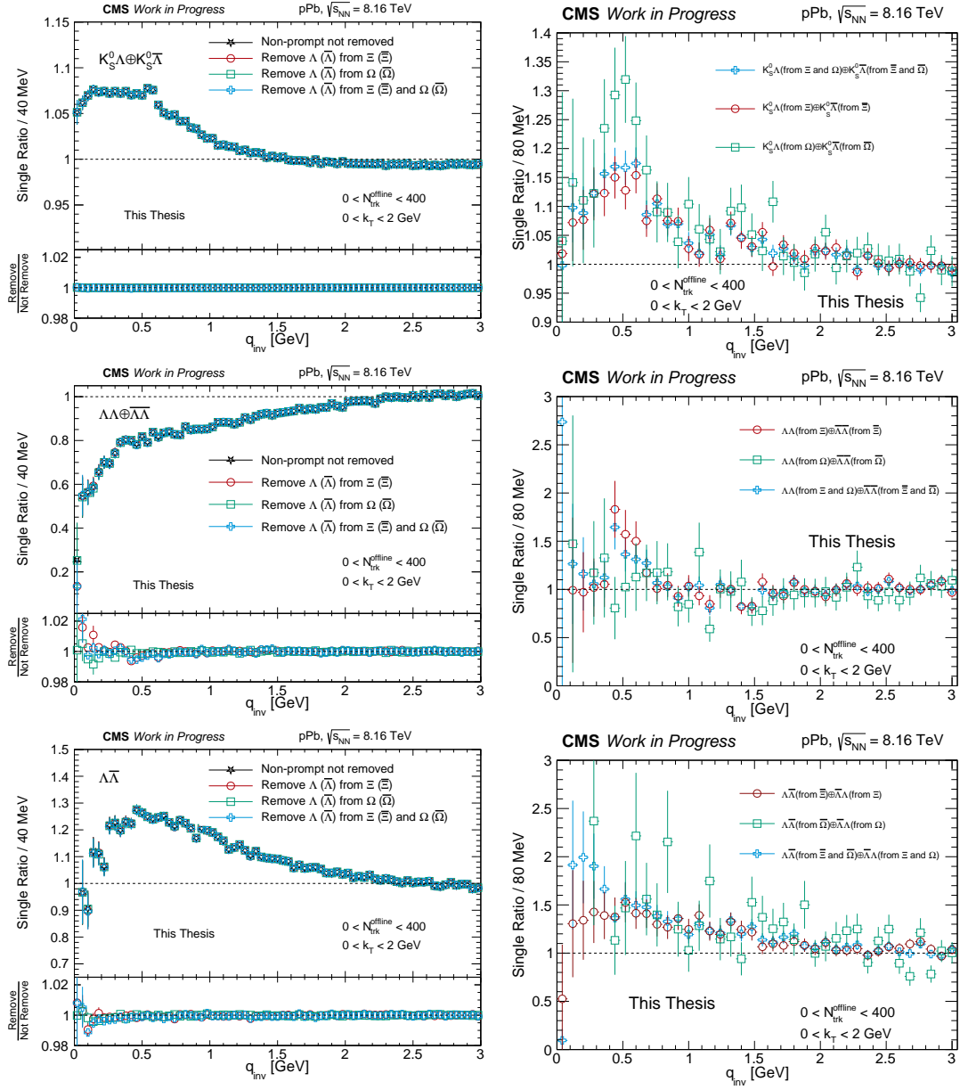
Figure 5.26: Single ratio plots for K_S^0\Lambda \oplus K_S^0\bar{\Lambda} (top panel), \Lambda\Lambda \oplus \bar{\Lambda}\bar{\Lambda} (middle panel) and \Lambda\bar{\Lambda} (bottom panel) integrated in k_T and N_{\text{trk}}^{\text{offline}} . Left panel: comparison of the correlations with (in different cases) and without the non-prompt removal. In the lower plot, the ratio between the distribution removing, cases ii), iii) and iv), and not removing, case i), the non-prompt contribution are shown. Right panel: correlation between prompt particles and non-prompt lambdas (from \Xi , \Omega and \Xi + \Omega ). The SR is rebinned to 80 MeV because of the lack of statistics. More informations at the text.
