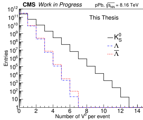
Figure 5.4: Number of V^0 's per event for K_S^0 (black solid line), \Lambda (blue dashed-dotted line) and \bar{\Lambda} (red dashed line) produced in pPb collisions using all MB and HM datasets. The first bin represent events with no V^0 candidates. More details in the text.
