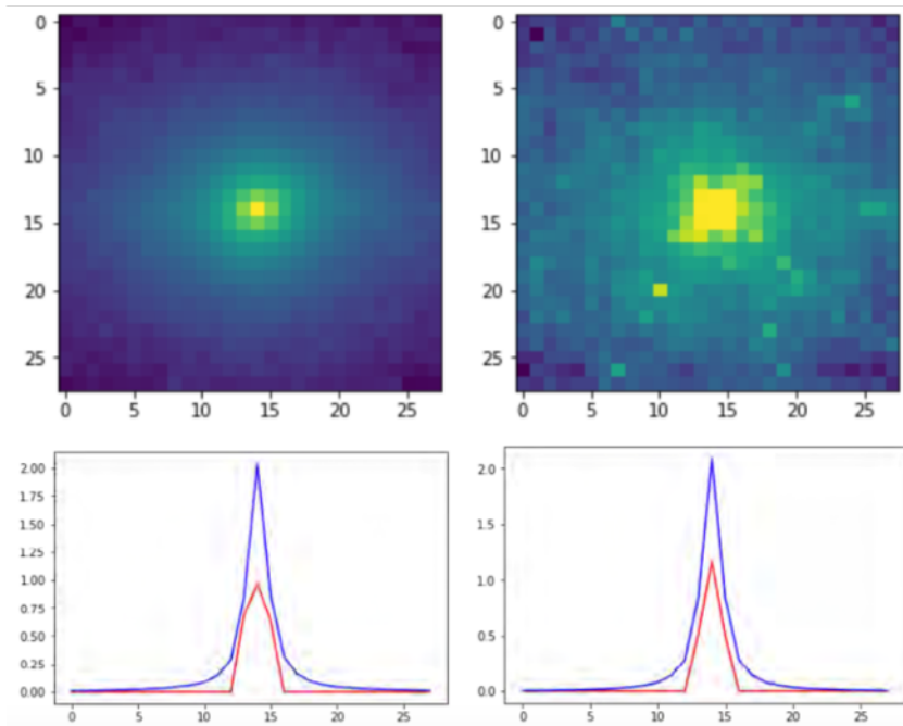
Figura 7: Interaction of a 50 GeV negative pion with the CMS ECAL barrel. Top: true (left) and synthetic (right) signals. Bottom: signal dispersion in \eta and \phi directions, for real (blue) and synthetic (red) signals.
